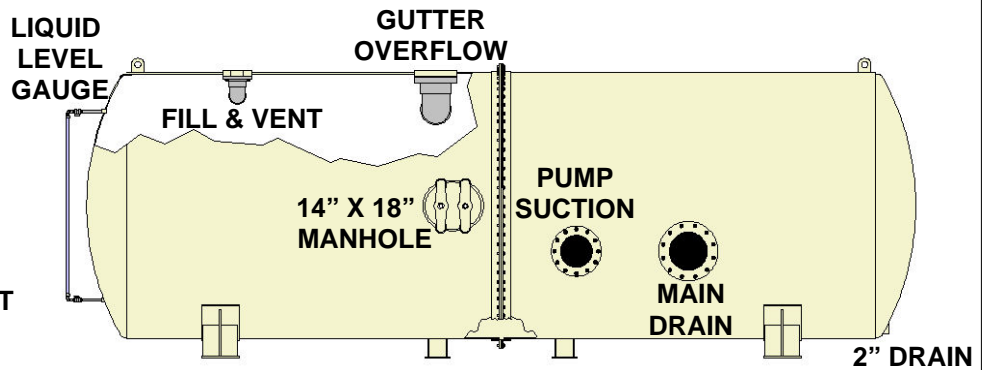
Steel or Fiberglass Horizontal Balancing Tanks
