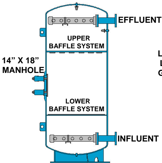
Fiberglass Contact Vessels
