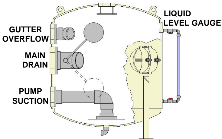
Steel Balancing Tanks
