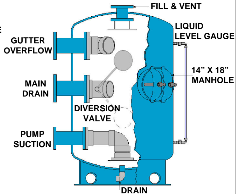
Fiberglass Balancing Tanks
